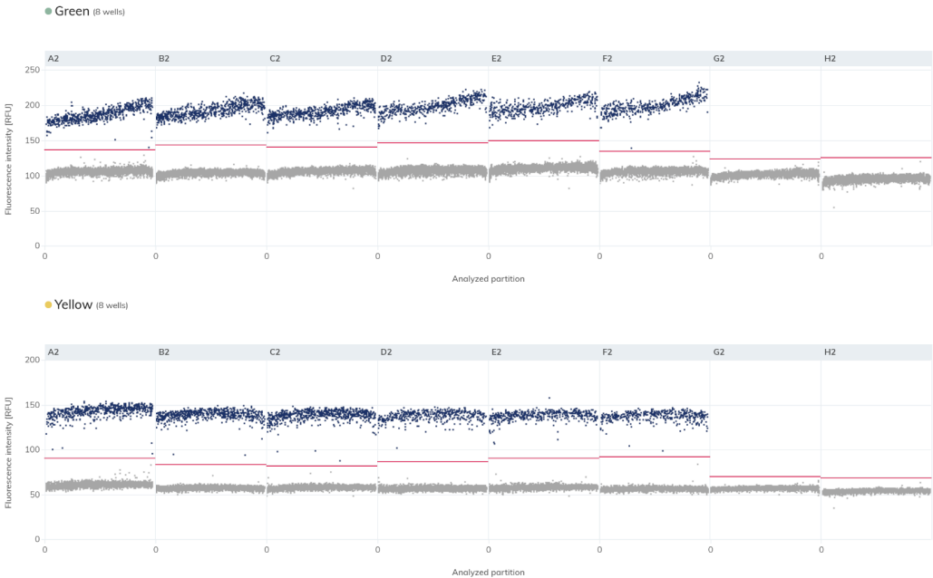
Figure 1. 1D Scatter Plot. Single-well data of target assay STK3 (Green Channel) and reference assay TERT (Yellow Channel) in different gDNA input amounts (A2, B2, C2: 6 ng/rxn; D2, E2, F2: 4 ng/rxn; G2, H2: NTCs).
