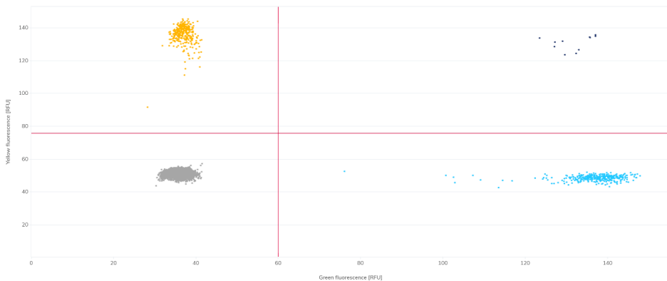
Figure 2. 2D Scatter Plot. Single-well data of target assay AKT1 (Green Channel, X-axis) and reference assay TERT (Yellow Channel, Y-axis) in 4 ng gDNA input amount.
