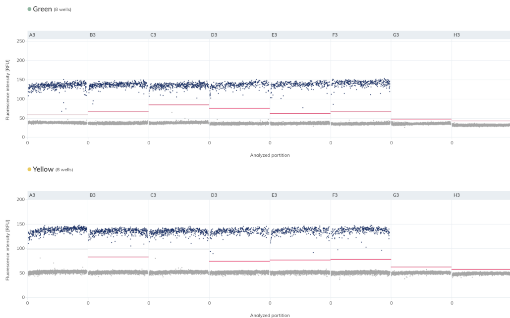
Figure 1. 1D Scatter Plot. Single-well data of target assay AKT1 (Green Channel) and reference assay TERT (Yellow Channel) in different gDNA input amounts ( A3, B3, C3 : 6 ng/rxn; D3, E3, F3 : 4 ng/rxn; G3, H3 : NTCs).
